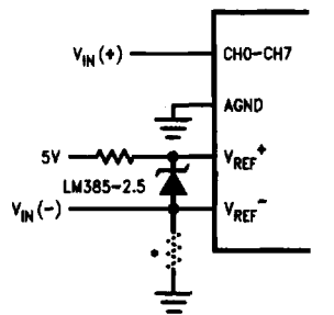
Input Not Referred to GND
