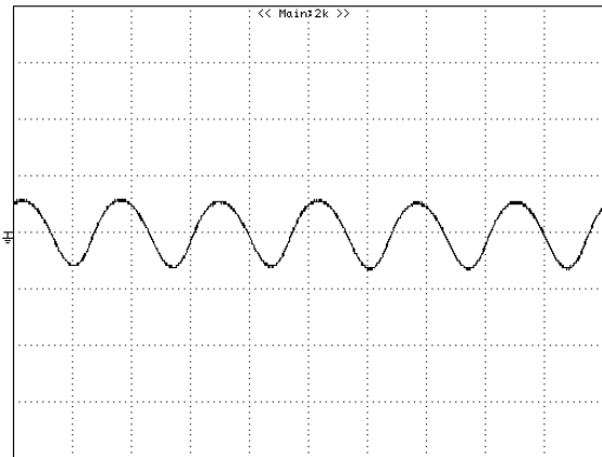
Figure 9: Input Terminal Ripple Current, i_c , at full rated output current and nominal input voltage ( V_{in}=48v ) with 12\mu H source impedance and 33\mu F electrolytic capacitor (200 mA/div, 1us/div)
