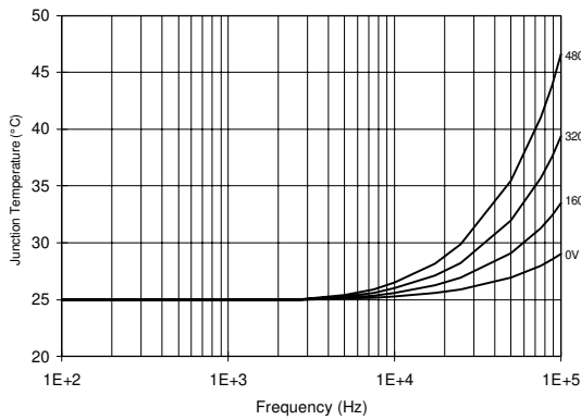
Figure 51. IR2130/IR2132 T J vs. Frequency (IRF820) R GATE = 33Ω, V CC = 15V
