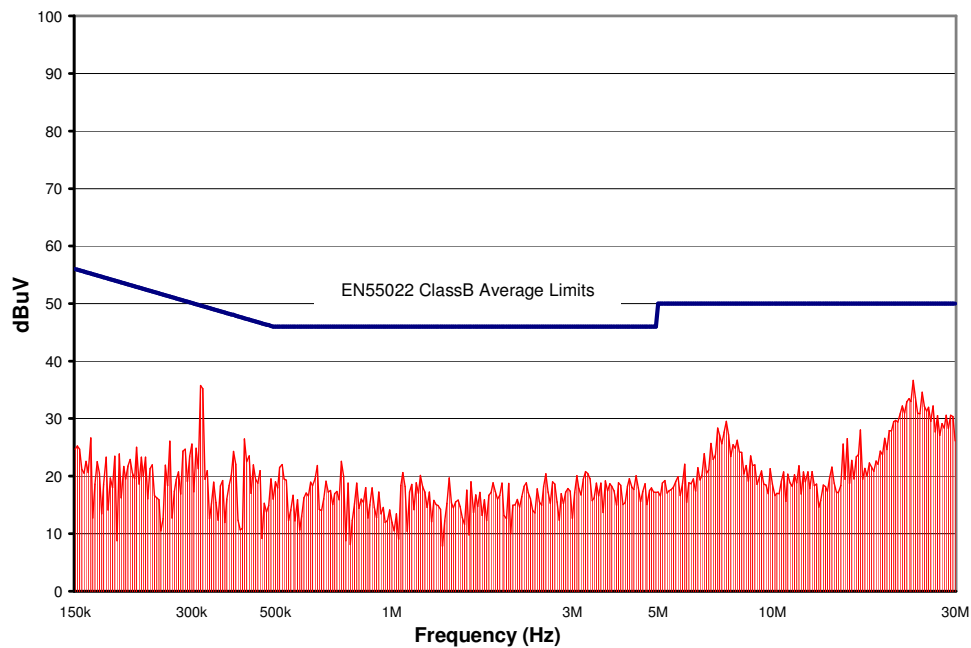
Figure 16. CPE6D24 Conducted Emissions using above specified input filter, Vin = 48V, Full Resistive Load
