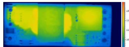
Thermal Image of module @ 24Vin, 200LFM & 40C
