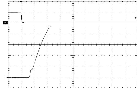
Figure 8. Startup Waveform via Enable Pin, time scale 10mS/div. Vin=Vin_nom, full resistive load + 1000uF (negative enable.) Ch1,Ch2=5V/div
