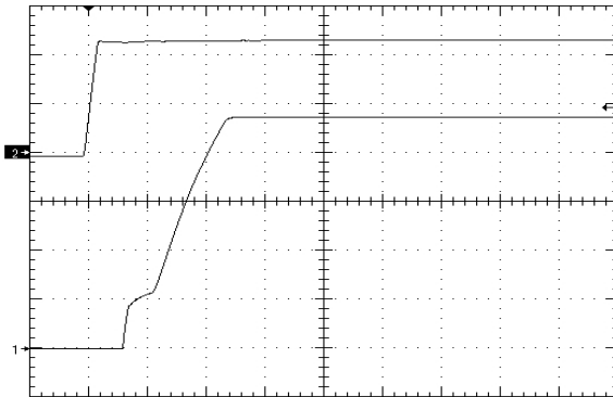
Figure 7. Startup Waveform via Line Voltage, time scale 10mS/div. Vin=Vin_nom, no load Ch1=5V/div, Ch2=10V/div
