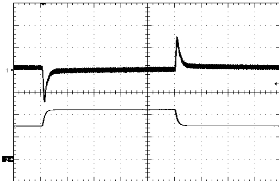
Figure 9. Load Transient Response (100mV/div), di/dt=0.1A/uS, 50% - 75% - 50% of full load, time scale: 200uS/div. Ch2=2A/div
