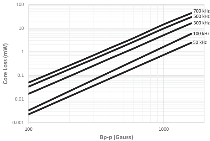
HCM1A4020V2-150-R
