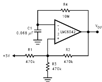
Figure 42. 1 Hz Square Wave Oscillator
