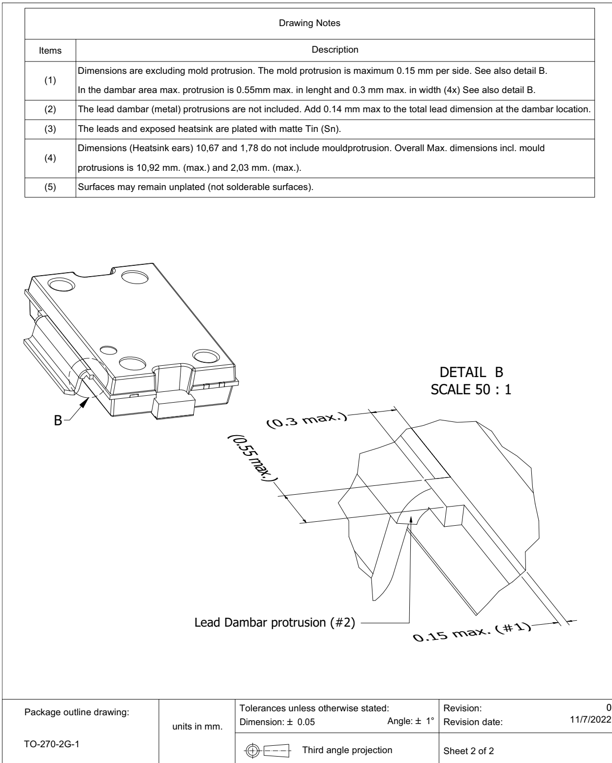
Fig 20. Package outline TO-270-2G-1 (sheet 2 of 2)
