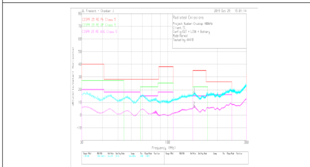
V_{OUT} = 5\text{ V} F_{SW} = 400\text{ kHz} I_{OUT} = 5\text{ A} Frequency tested: 30 MHz to 300 MHz Tested on 6-A variant with LM61460EVM
