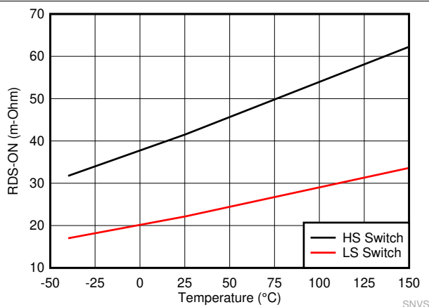
Figure 7-5. High-Side and Low-Side Switches R_{DS\_ON}
