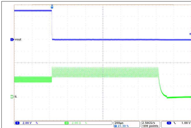
V_{OUT} = 5\text{ V} F_{SW} = 2100\text{ kHz} FPWM mode I_{OUT} = 3\text{ A to Short Circuit} V_{IN} = 13.5\text{ V}
