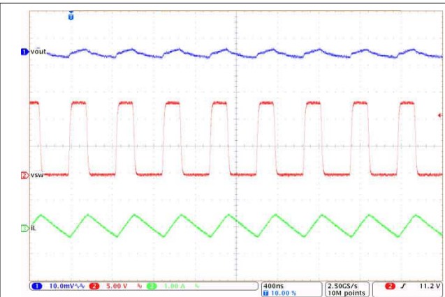
V_{OUT} = 5\text{ V} F_{SW} = 2100\text{ kHz} FPWM mode I_{OUT} = 100\text{ mA} V_{IN} = 13.5\text{ V}
