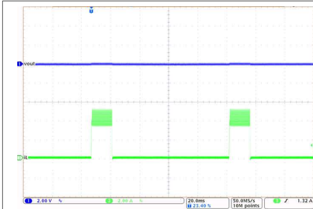
Figure 8-12. Inductor Current Bursts During Hiccup
