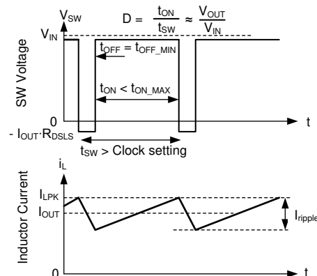
Figure 8-19. Frequency and Output Voltage in Dropout
