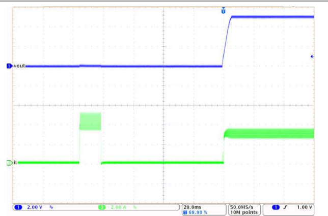
Figure 8-13. Short-Circuit Recovery
