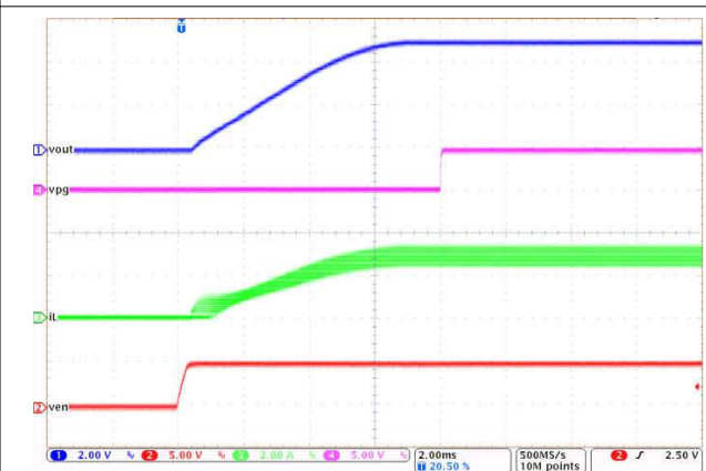
V_{OUT} = 5\text{ V} F_{SW} = 2100\text{ kHz} FPWM mode I_{OUT} = 3\text{ A} V_{IN} = 13.5\text{ V}
