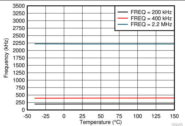
Figure 7-4. Switching Frequency Set by RT Resistor
