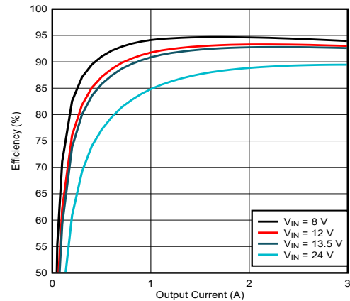
Figure 9-11. LM61430-Q1 Efficiency
