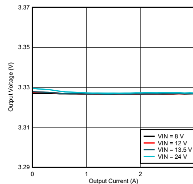
Figure 9-15. LM61430-Q1 Load and Line Regulation
