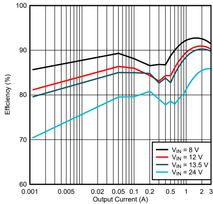
Figure 9-4. LM61430-Q1 Efficiency
