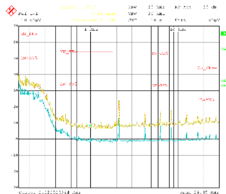
Conducted EMI: V_{OUT} = 5\text{ V} , F_{SW} = 210\text{ kHz}
