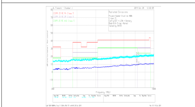
V_{OUT} = 5\text{ V} F_{SW} = 400\text{ kHz} I_{OUT} = 5\text{ A} Frequency tested: 300 MHz to 1 GHz Tested on 6-A variant with LM61460EVM
