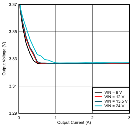
Figure 9-12. LM61430-Q1 Load and Line Regulation
