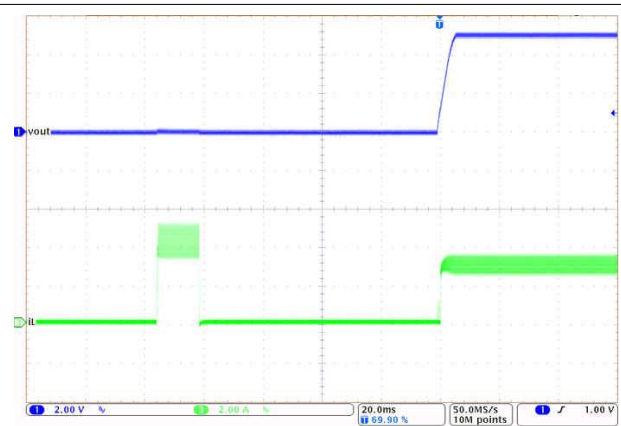
V_{OUT} = 5\text{ V} F_{SW} = 2100\text{ kHz} FPWM mode I_{OUT} = \text{Short Circuit to } 3\text{ A} V_{IN} = 13.5\text{ V}
