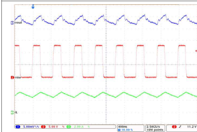
V_{OUT} = 5\text{ V} F_{SW} = 2100\text{ kHz} Auto mode I_{OUT} = 3\text{ A} V_{IN} = 13.5\text{ V}
