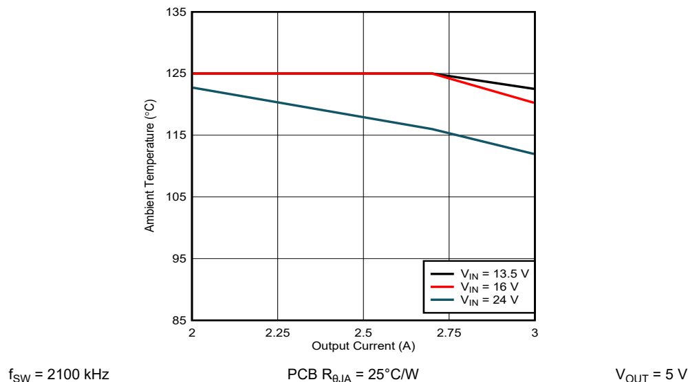
Figure 9-2. Maximum Ambient Temperature versus Output Current
