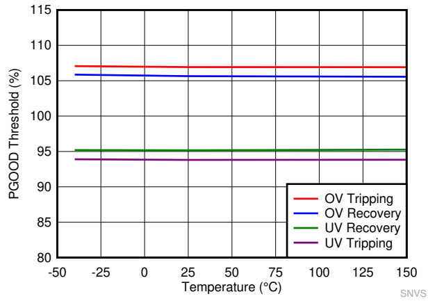
Figure 7-7. PGOOD Thresholds
