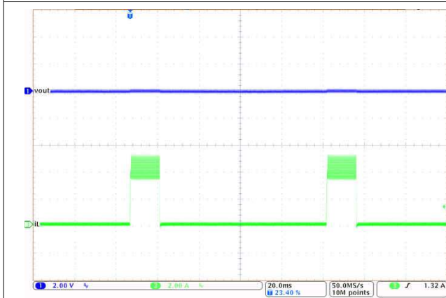
V_{OUT} = 5\text{ V} F_{SW} = 2100\text{ kHz} FPWM mode I_{OUT} = \text{Short Circuit} V_{IN} = 13.5\text{ V}
