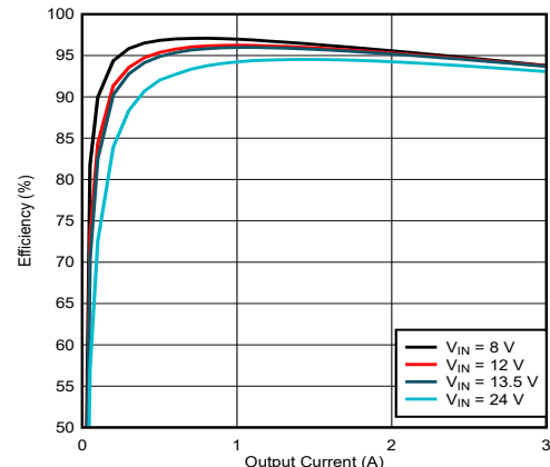
Figure 9-7. LM61430-Q1 Efficiency
