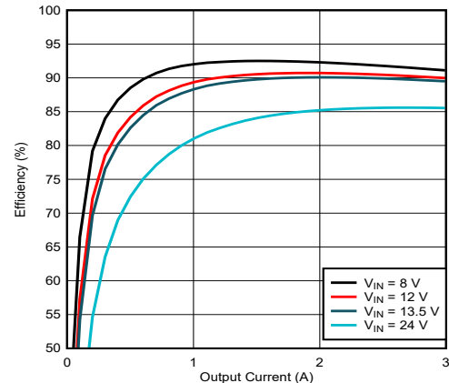
Figure 9-5. LM61430-Q1 Efficiency
