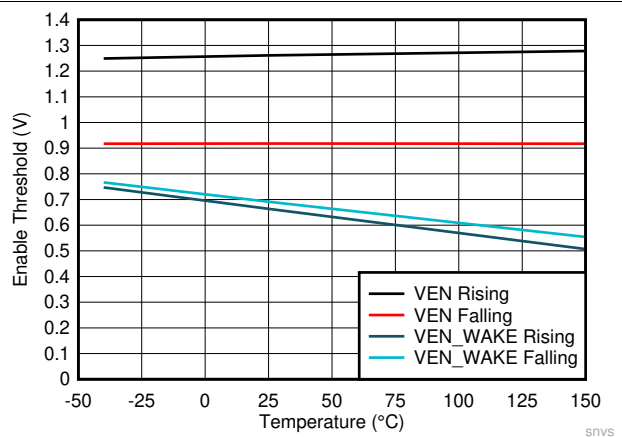
Figure 7-6. Enable Thresholds
