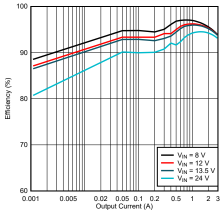
Figure 9-6. LM61430-Q1 Efficiency
