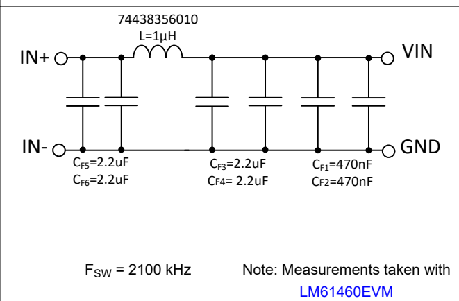
Figure 9-45. Recommended Input EMI Filter
