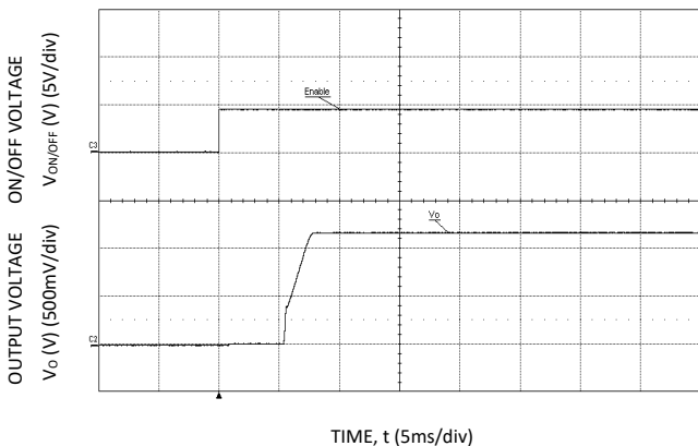
Figure 11. Typical Start-up Using On/Off Voltage (Io = Io,max, Vin=12V,Cext= 22uF).
