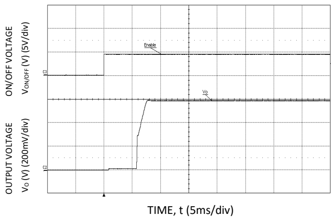
Figure 5. Typical Start-up Using On/Off Voltage (Io = Io,max, Vin=12V,Cext= 22µF).
