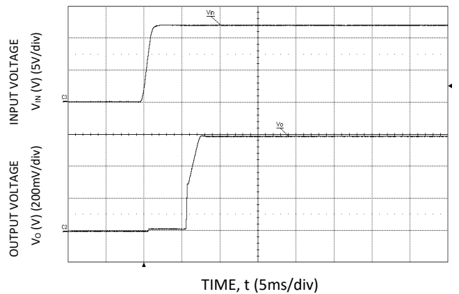
Figure 6. Typical Start-up Using Input Voltage (VIN = 12V, Cext= 22µF ,Io = Io,max).
