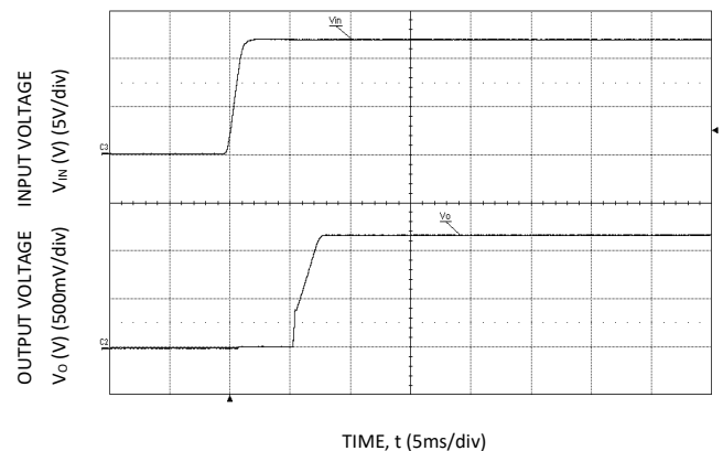
Figure 12. Typical Start-up Using Input Voltage (VIN = 12V, Cext= 22uF, Io = Io,max).
