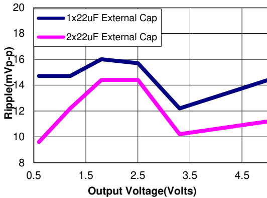
Figure 5. Output ripple voltage for various output voltages with external 1x22 μF, 2x22 μF ceramic capacitors at the output (2A load). Input voltage is 12V.
