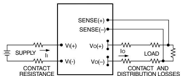
Figure 24. Effective Circuit Configuration for Single-Module Remote-Sense Operation
