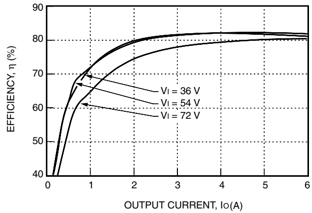
Figure 12. JW030A-M Typical Converter Efficiency vs. Output Current
