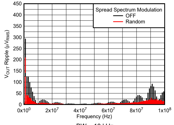
BW = 10 kHz 12 V to 1.2 V, 1 A 2.2 \mu\text{H} , 1 MHz First L-C Only Figure 6-2. V_{OUT} Ripple FFT After the First L-C Filter
