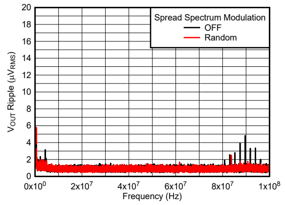
BW = 10 kHz 5 V to 3.3 V, 1 A 2.2 \mu\text{H} , 2.2 MHz First and second L-C Figure 6-24. V_{OUT} Ripple FFT After the Second L-C Filter
