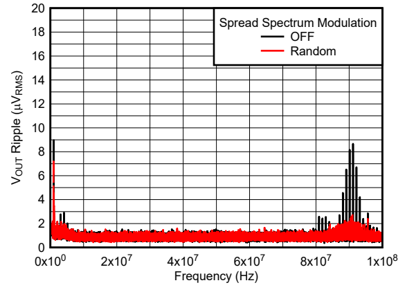
BW = 10 kHz 12 V to 1.2 V, 1 A 2.2 \mu\text{H} , 1 MHz First and second L-C Figure 6-4. V_{OUT} Ripple FFT After the Second L-C Filter
