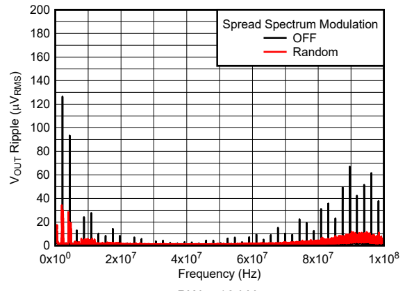
BW = 10 kHz 5 V to 3.3 V, 1 A 2.2 \mu\text{H} , 2.2 MHz First L-C Only Figure 6-22. V_{OUT} Ripple FFT After the First L-C Filter
