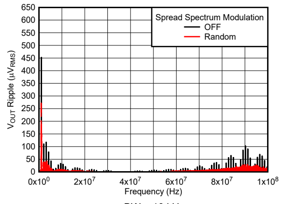
BW = 10 kHz 12 V to 1.8 V, 1 A 2.2 \mu\text{H} , 1 MHz First L-C Only Figure 6-6. V_{OUT} Ripple FFT After the First L-C Filter
