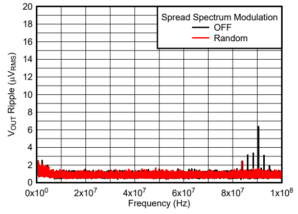
BW = 10 kHz 5 V to 1.8 V, 1 A 2.2 \mu\text{H} , 2.2 MHz First and second L-C Figure 6-20. V_{OUT} Ripple FFT After the Second L-C Filter
