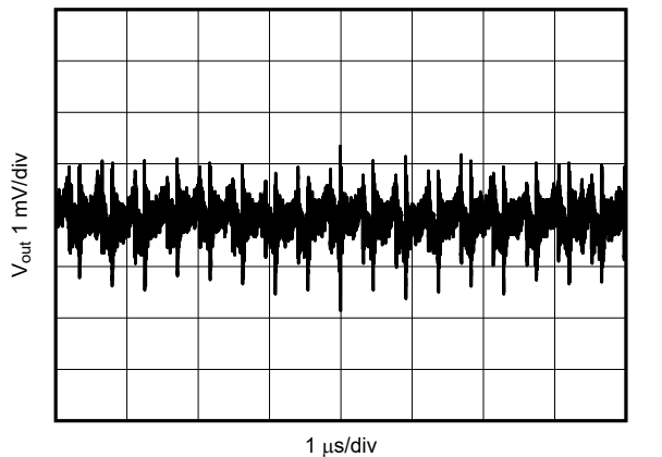
5 V to 3.3 V, 1 A 2.2 \mu\text{H} , 2.2 MHz First L-C Only Figure 6-21. V_{OUT} Ripple After the First L-C Filter
