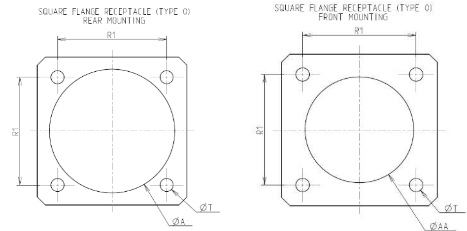
Panel Cutout
