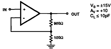
FIGURE 1. TEST CIRCUIT
