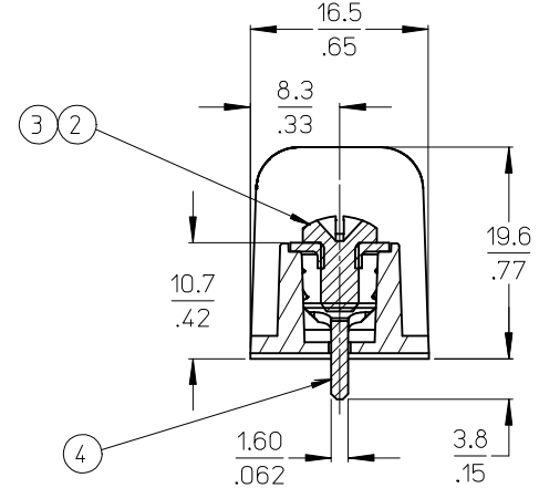
SECTION Z-Z
