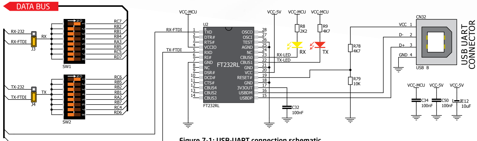
Figure 7-1: USB-UART connection schematic
