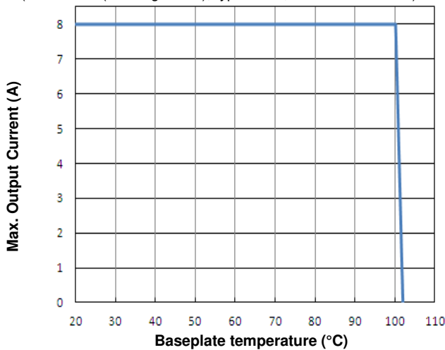
Figure 11. Current Derating Curve for Baseplate
