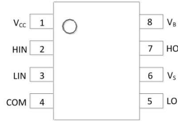
Top View: SO-8
