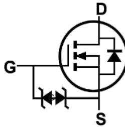
Equivalent Circuit
