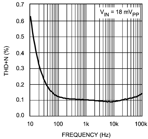
Total Harmonic Distortion vs. Frequency (LMV1012-07)
