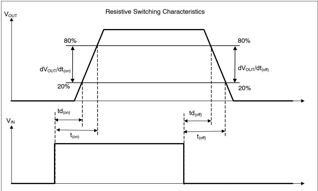
Figure 4. Switching Characteristics
