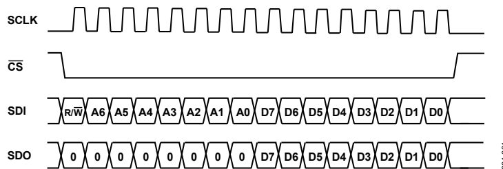
Figure 80. Write/Read Command
