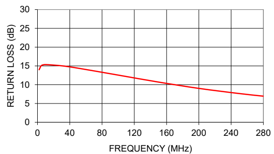
RETURN LOSS
