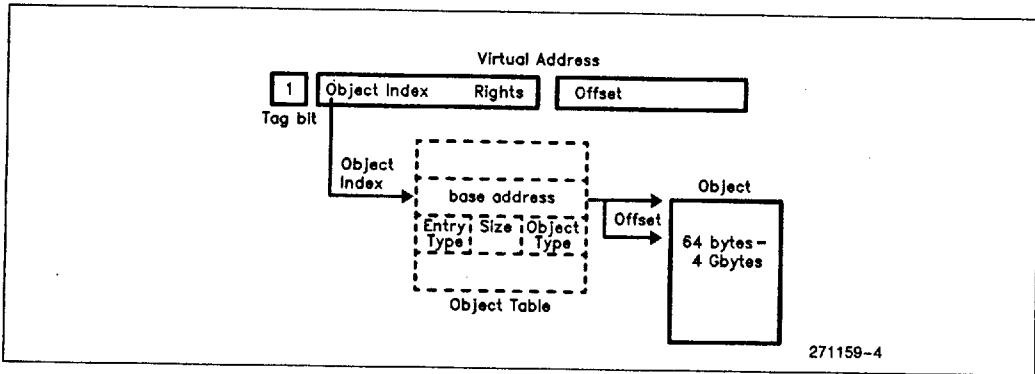
Figure 6. Virtual Addressing
