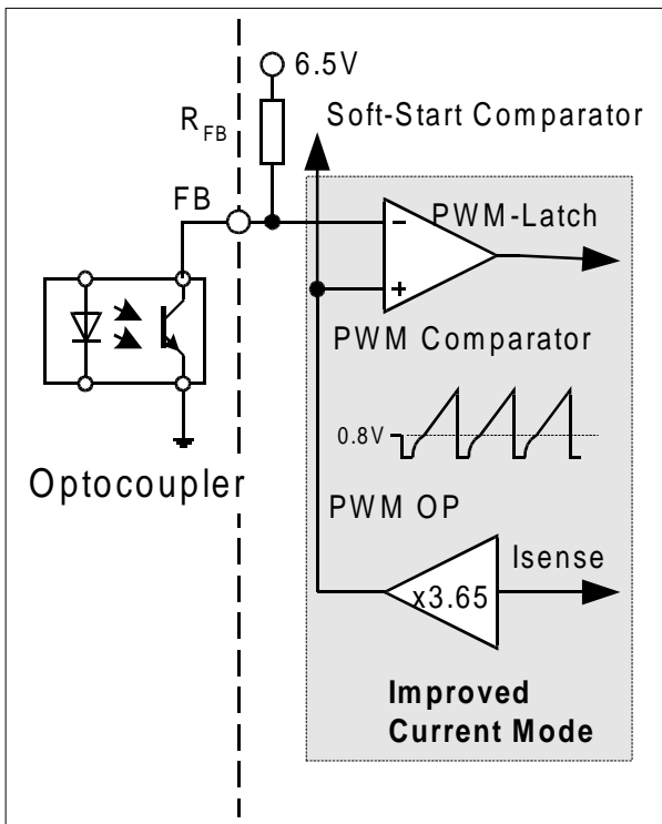
Figure 8 PWM Controlling
