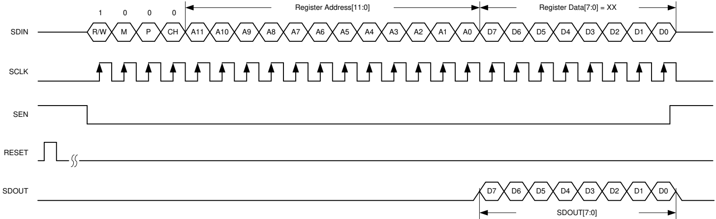
Figure 7-21. Serial Register Read Timing Diagram
