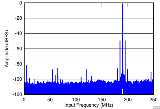
Figure 6-40. Power-Supply Rejection Ratio FFT for Test Signal on AVDD Supply
