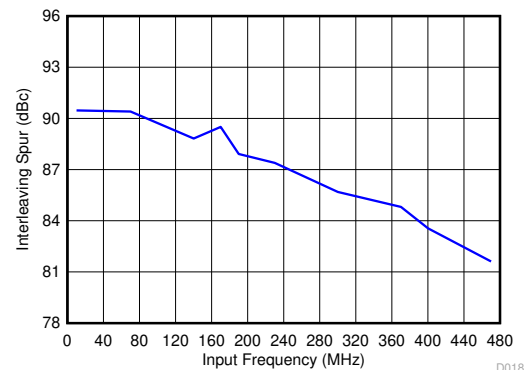
Figure 6-20. IL Spur vs Input Frequency
