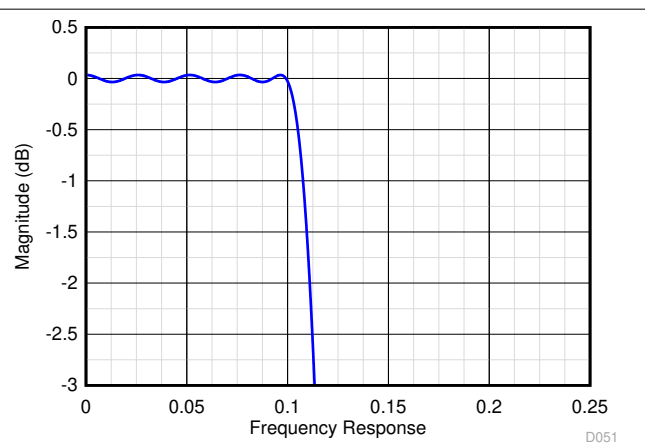
Figure 7-11. Zoomed View of Frequency Response
