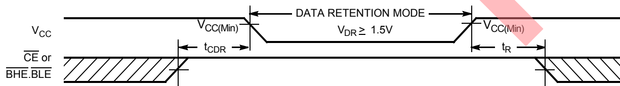
Figure 3. Data Retention Waveform [7]
