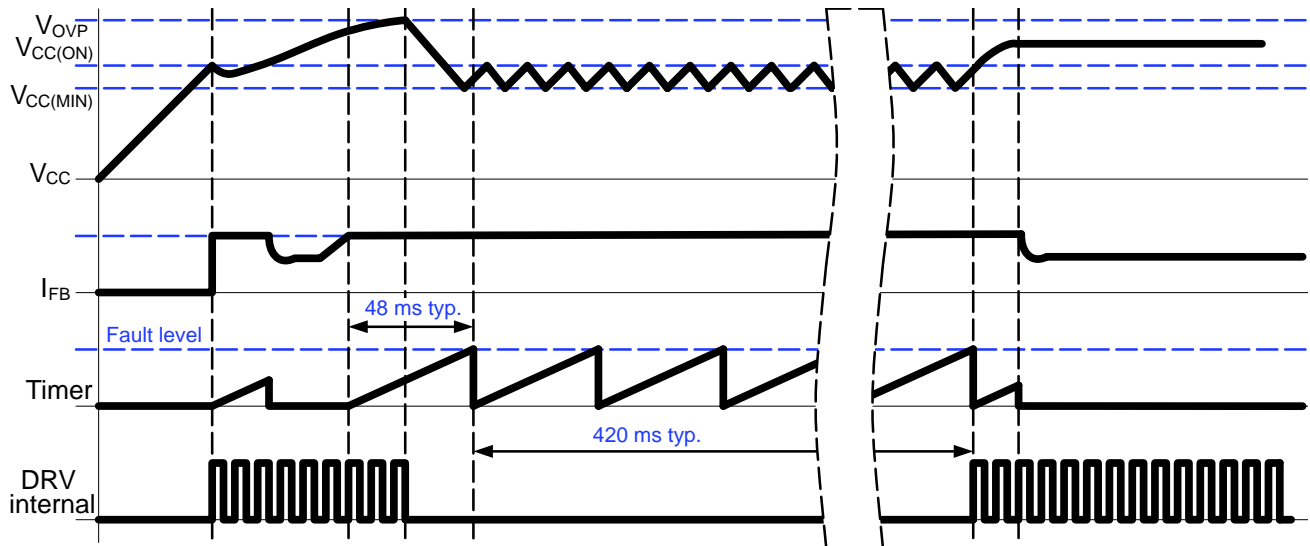
Figure 38. Describes the Main Signal Variations When the Part Operates in Auto-recovery OVP
