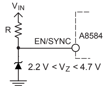
Figure 4. Automatically enabling the A8584 from V_{IN} or some other power rail
