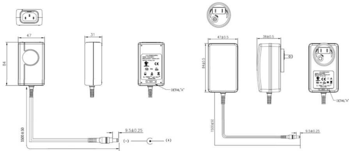
IEC60320 C14 Receptacle, 2.5mm x 5.5mm x 9.5mm Barrel Connector Interchangeable N.A. Blade, 2.5mm x 5.5mm x 9.5mm Barrel Connector
