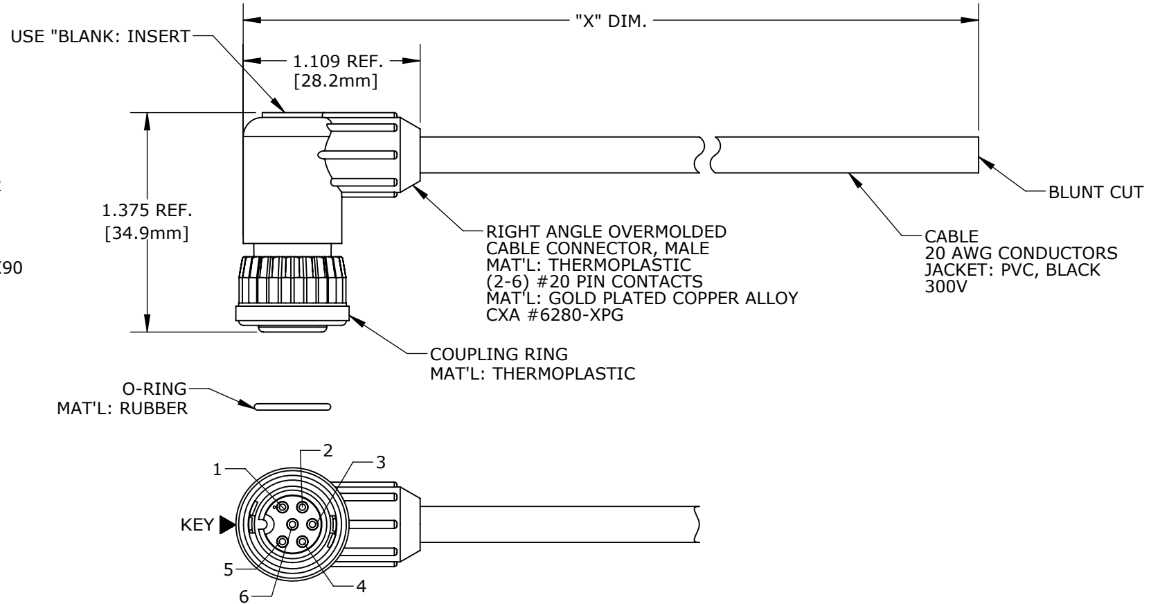
END "A" FACE VIEW SHOWN CARA62806PXXX90
