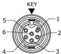
FACE VIEW P/N: CARA62806PXXX90
