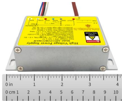
Figure 1.3. Side View
