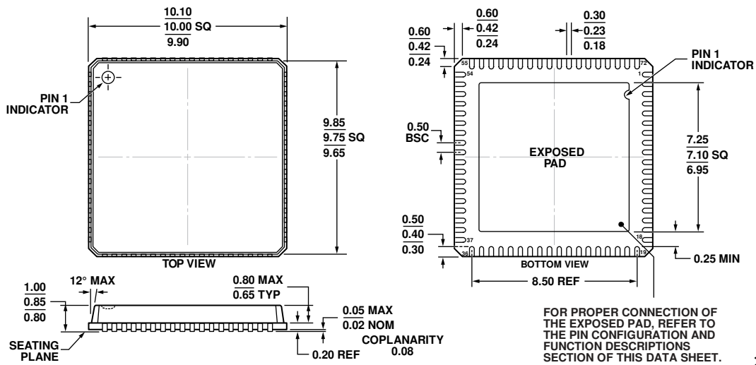
Figure 57. 72-Lead Lead Frame Chip Scale Package [LFCSP_VQ] 10 mm × 10 mm Body, Very Thin Quad (CP-72-4) Dimensions shown in millimeters
