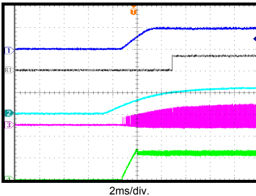
Start-Up through Input Voltage I_{OUT}=12A
