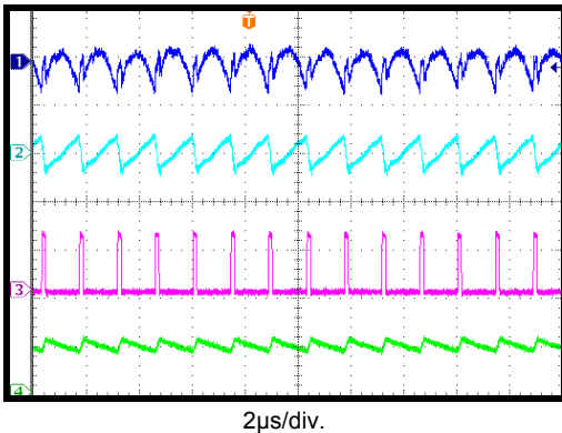
Input/Output Ripple I_{OUT}=12A
