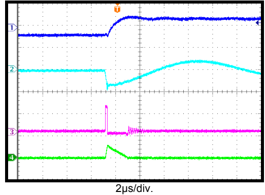
Input/Output Ripple I_{OUT}=0A
