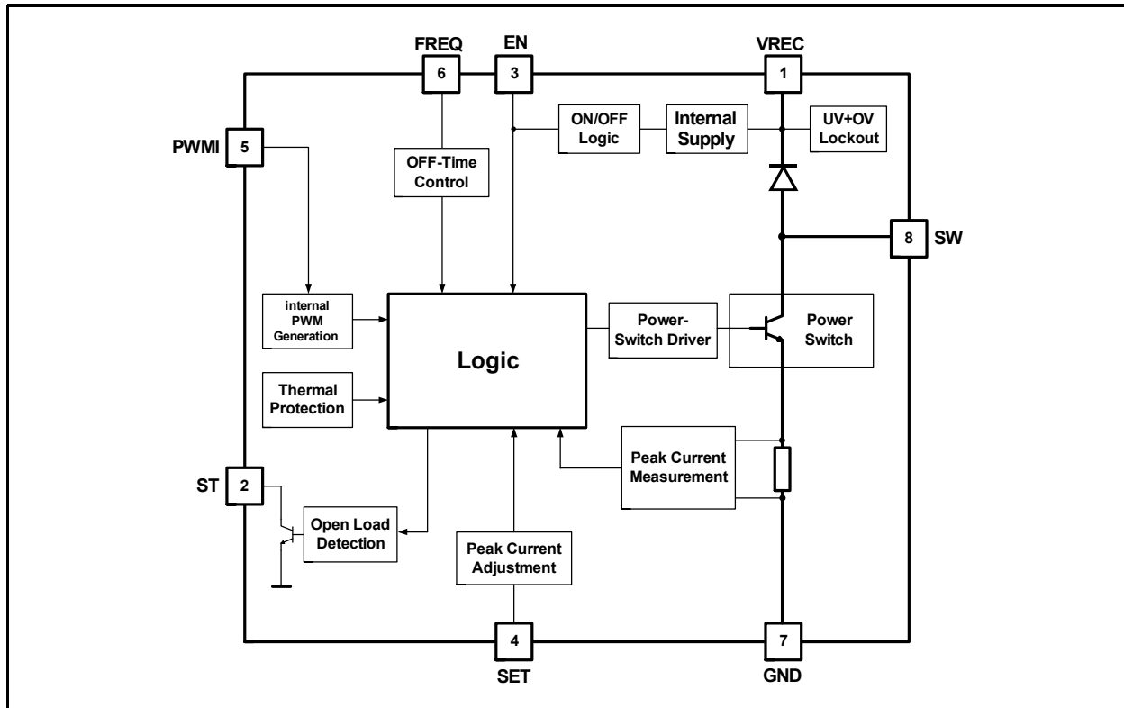
Figure 2-1 Block Diagram TLD5045EJ
