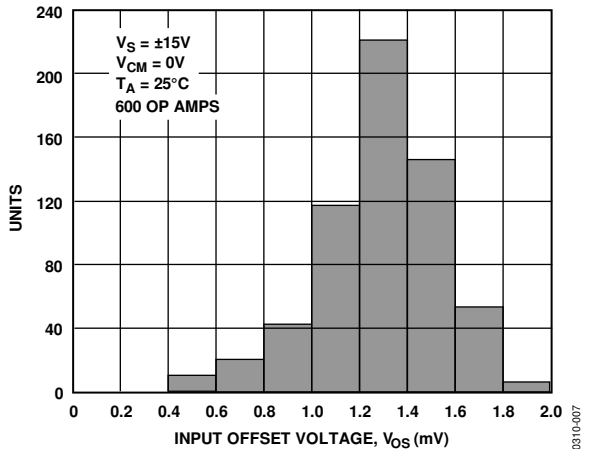
Figure 7. OP492 Input Offset Voltage Distribution @ \pm 15\text{V}
