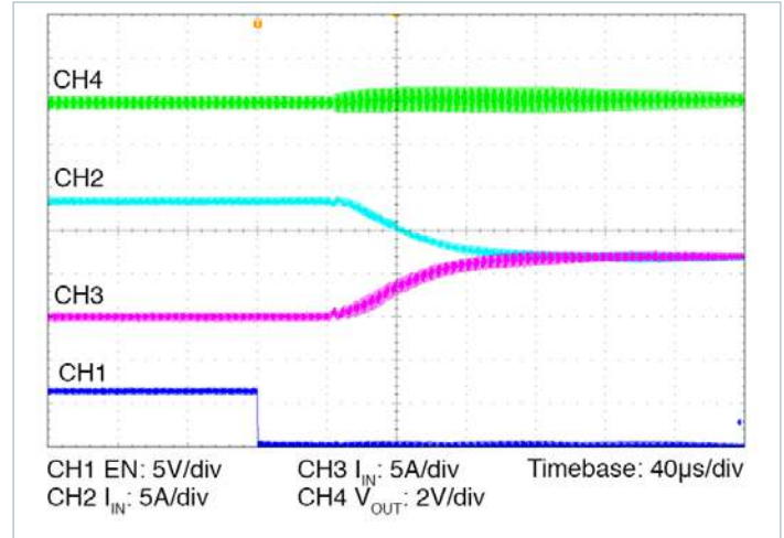
Figure 19 — Two modules parallel array test. V_{OUT} and I_{IN} change when one module is enabled. Nominal V_{IN} , I_{OUT} = 53A
