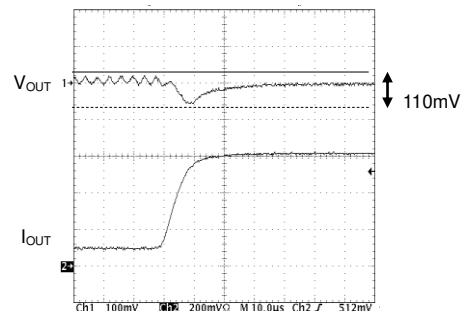
BD9106FVM-LB (Load response I_O=100mA \rightarrow 600mA )
