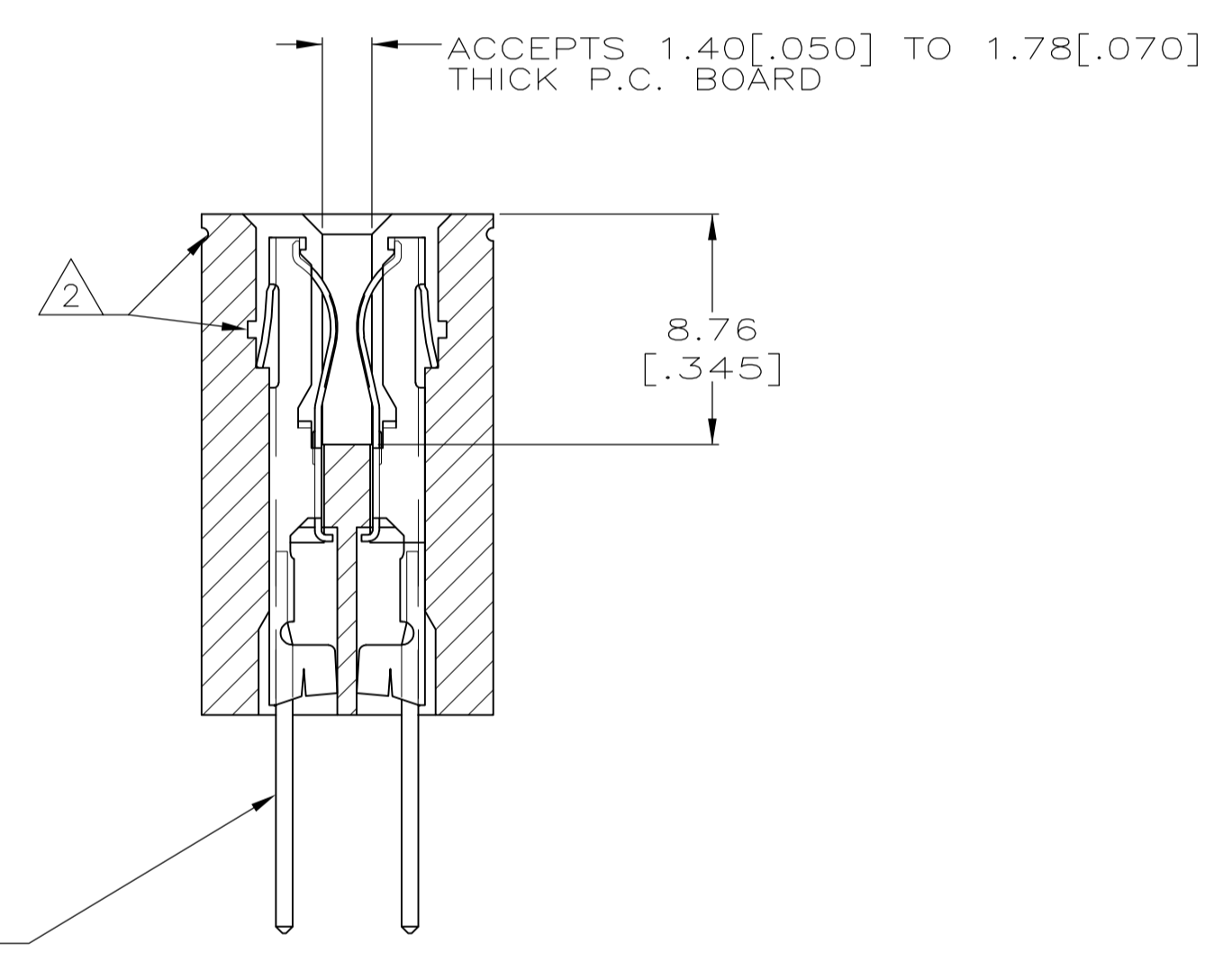
SECTION Z-Z
