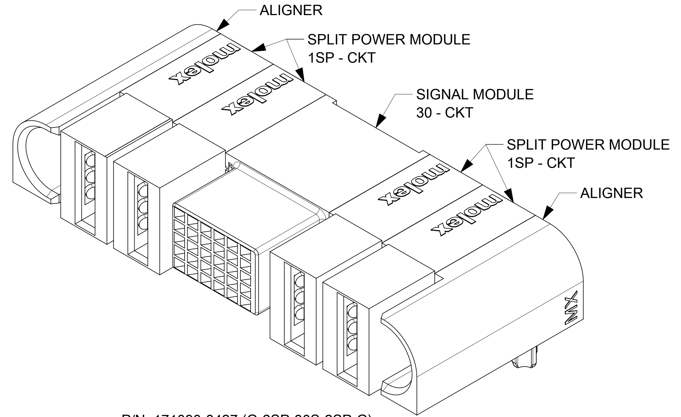
P/N: 171090-8427 (G-2SP-30S-2SP-G)
