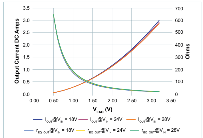
Figure 103 — r_{EQ\_OUT} vs. output current vs. V_{EAO} , V_{OUT} = 50\text{V} ; 18 – 28 V_{IN}
