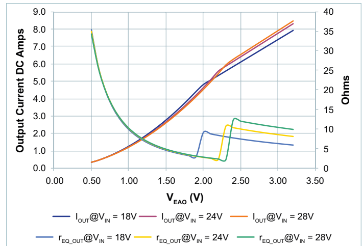
Figure 67 — r_{EQ\_OUT} vs. Output Current vs. V_{EAO} , V_{OUT} = 10V ; 18 - 28V_{IN}
