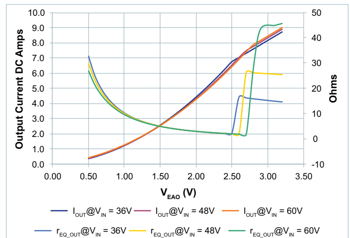
Figure 68 — r_{EQ\_OUT} vs. output current vs. V_{EAO} , V_{OUT} = 10V ; 36 - 60V_{IN}
