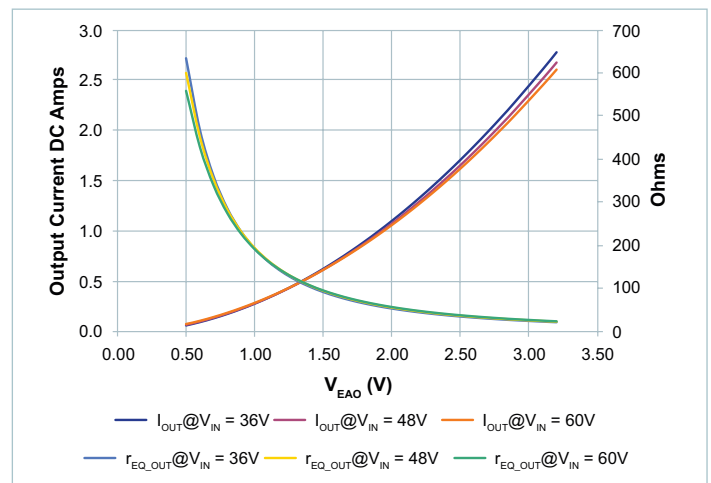
Figure 104 — r_{EQ\_OUT} vs. output current vs. V_{EAO} , V_{OUT} = 50\text{V} ; 36 – 60 V_{IN}
