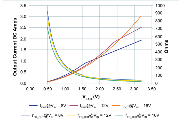
Figure 102 — r_{EQ\_OUT} vs. output current vs. V_{EAO} , V_{OUT} = 50\text{V} ; 8 – 16 V_{IN}
