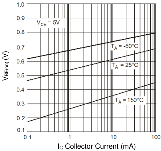
Figure 6. V_{BE(on)} v I_C
