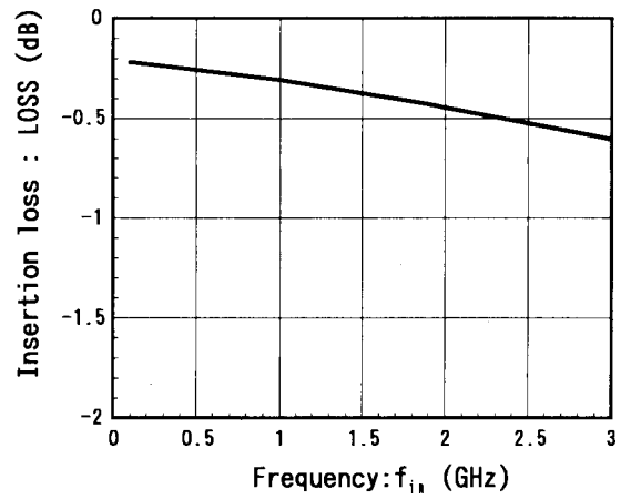
(PC-P2) Insertion loss vs. Frequency
