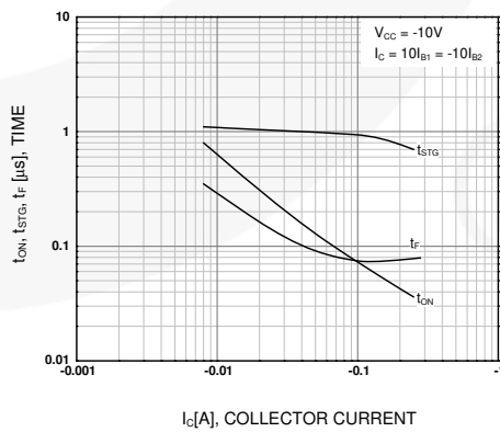
Figure 6. Switching Time
