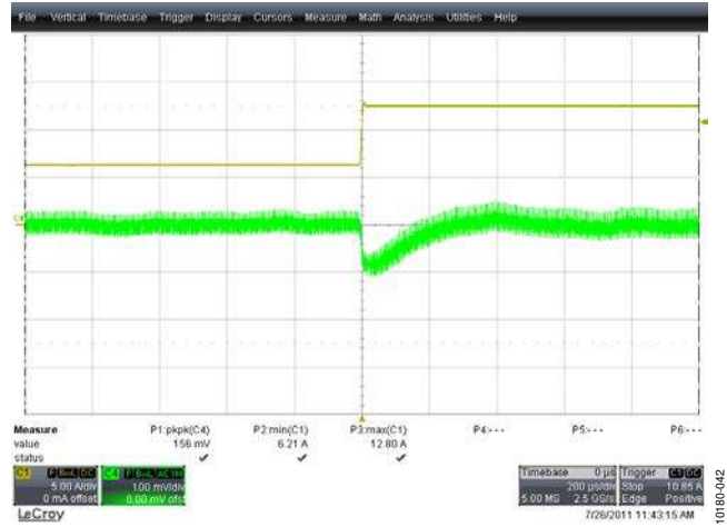
Figure 43. Output Voltage Transient, 25% to 50% Load, 385 V DC, One Phase Only Yellow Trace: Load Current, 5 A/div, 200 µs/div Green Trace: Output Voltage (AC-Coupled), 100 mV/div, 200 µs/div
