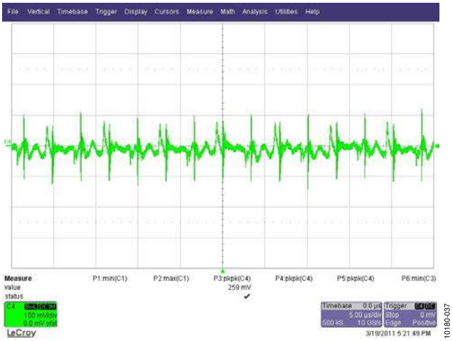
Figure 38. Output Voltage at 2700 μF Capacitor C10 (AC-Coupled), 385 V DC, 25 A, 100 mV/div, 5 μs/div, High Frequency Component
