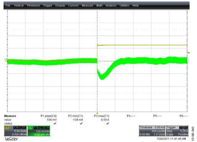
Figure 41. Output Voltage Transient, 0% to 25% Load, 385 V DC, One Phase Only Yellow Trace: Load Current, 5 A/div, 500 μs/div Green Trace: Output Voltage (AC-Coupled), 100 mV/div, 500 μs/div
