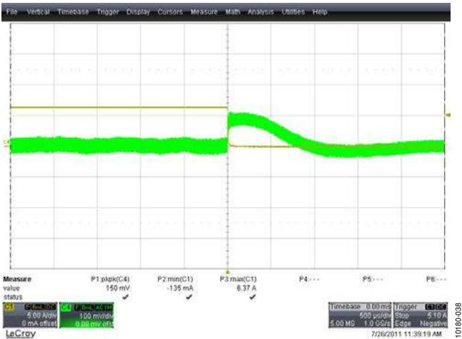
Figure 39. Output Voltage Transient, 25% to 0% Load, 385 V DC, One Phase Only Yellow Trace: Load Current, 5 A/div, 500 μs/div Green Trace: Output Voltage (AC-Coupled), 100 mV/div, 500 μs/div
