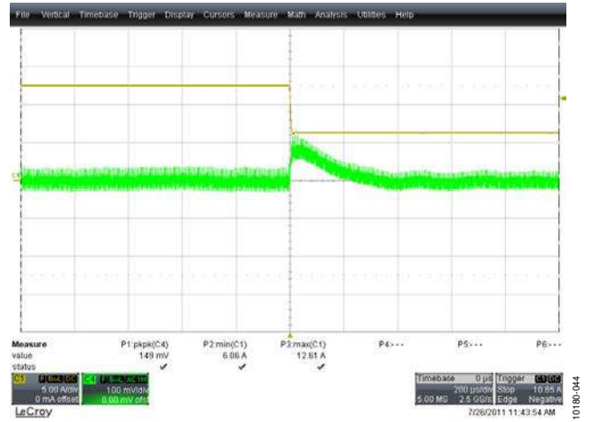
Figure 45. Output Voltage Transient, 50% to 25% Load, 385 V DC, One Phase Only Yellow Trace: Load Current, 5 A/div, 200 µs/div Green Trace: Output Voltage (AC-Coupled), 100 mV/div, 200 µs/div
