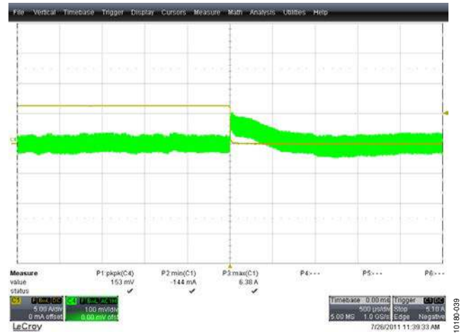
Figure 40. Output Voltage Transient, 25% to 0% Load, 385 V DC, Both Phases Active Yellow Trace: Load Current, 5 A/div, 500 μs/div Green Trace: Output Voltage (AC-Coupled), 100 mV/div, 500 μs/div
