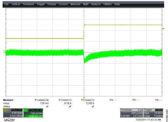
Figure 44. Output Voltage Transient, 25% to 50% Load, 385 V DC, Both Phases Active Yellow Trace: Load Current, 5 A/div, 200 µs/div Green Trace: Output Voltage (AC-Coupled), 100 mV/div, 200 µs/div
