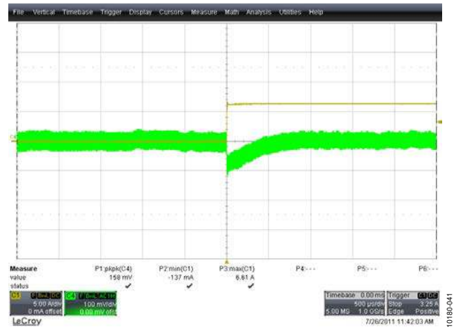
Figure 42. Output Voltage Transient, 0% to 25% Load, 385 V DC, Both Phases Active Yellow Trace: Load Current, 5 A/div, 500 μs/div Green Trace: Output Voltage (AC-Coupled), 100 mV/div, 500 μs/div
