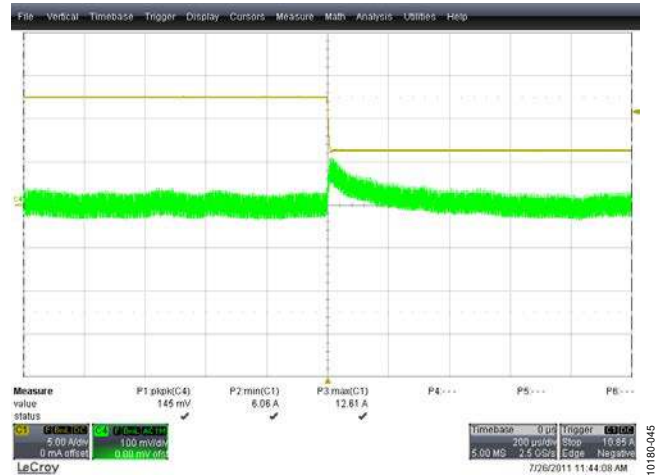
Figure 46. Output Voltage Transient, 50% to 25% Load, 385 V DC, Both Phases Active Yellow Trace: Load Current, 5 A/div, 200 µs/div Green Trace: Output Voltage (AC-Coupled), 100 mV/div, 200 µs/div
