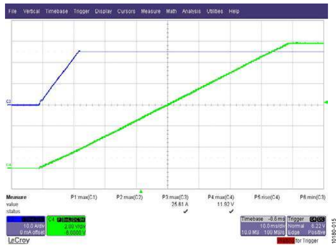
Figure 16. Startup at 350 V DC, 25 A Load (1 A/ \mu s Slew Rate) Green Trace: Output Voltage, 2 V/div, 10 ms/div Blue Trace: Load Current, 10 A/div, 10 ms/div
