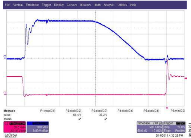
Figure 32. Synchronous Rectifier and Freewheeling MOSFET PIV at 25 A Load, 350 V DC Blue Trace: Synchronous Rectifier, 10 V/div, 500 ns/div Red Trace: Freewheeling FET Voltage, 20 V/div, 500 ns/div
