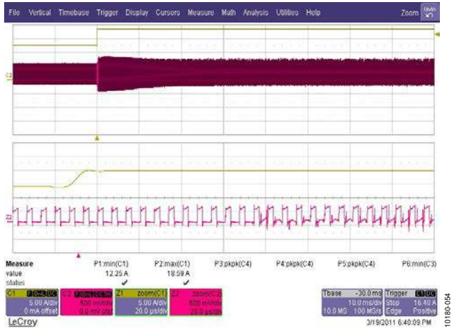
Figure 55. Input Current During Load Step of 10 A to 20 A Yellow Trace: Load Current, 5 A/div, 10 ms/div Red Trace: Voltage at CS1 Pin, 500 mV/div (20 \mu s/div Zoomed In)
