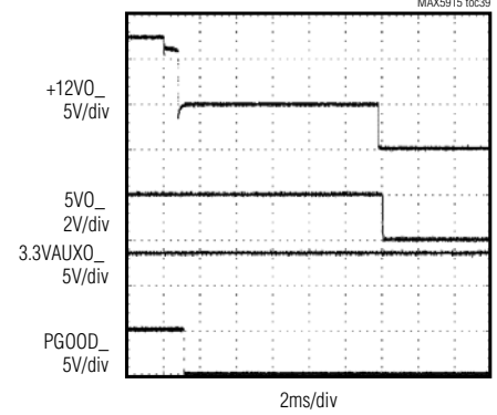
MAIN SUPPLY LATCHED FAULT MANAGEMENT
