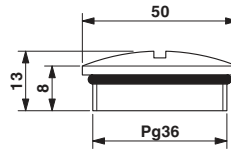
Filler plugs Pg36
