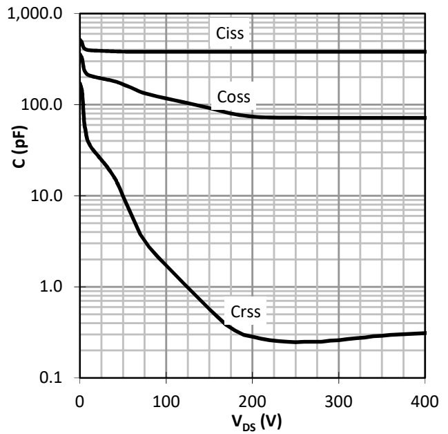
Figure 18 Typ. capacitances
