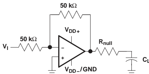
Figure 61. Series-Resistance Circuit
