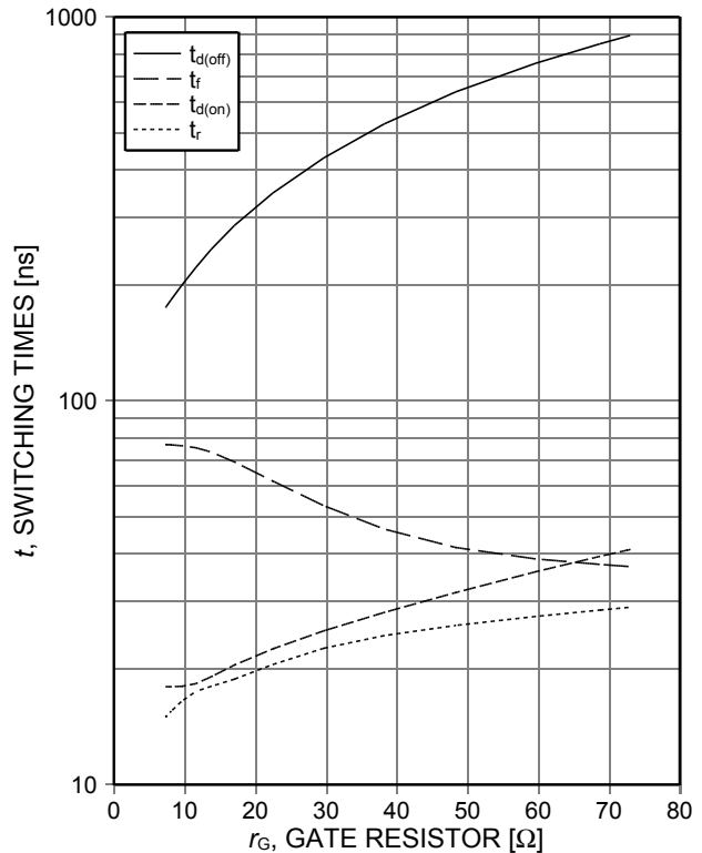
Figure 8. Typical switching times as a function of gate resistor (inductive load, T_j=175^\circ\text{C} , V_{CE}=400V , V_{GE}=0/15V , I_c=20A , Dynamic test circuit in Figure E)
