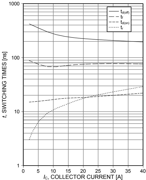
Figure 7. Typical switching times as a function of collector current (inductive load, T_j=175^\circ\text{C} , V_{CE}=400V , V_{GE}=0/15V , r_G=12\Omega , Dynamic test circuit in Figure E)
