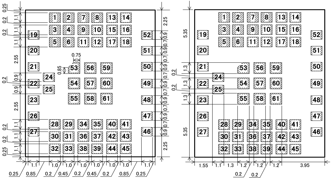
Recommended Board Land Pattern (Top View)
